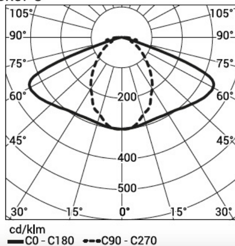
DROP S
