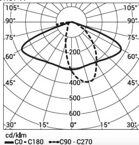
DROP A
