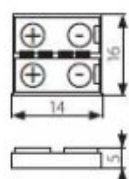
CONNECTOR RGB 10
