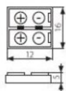
CONNECTOR 8
