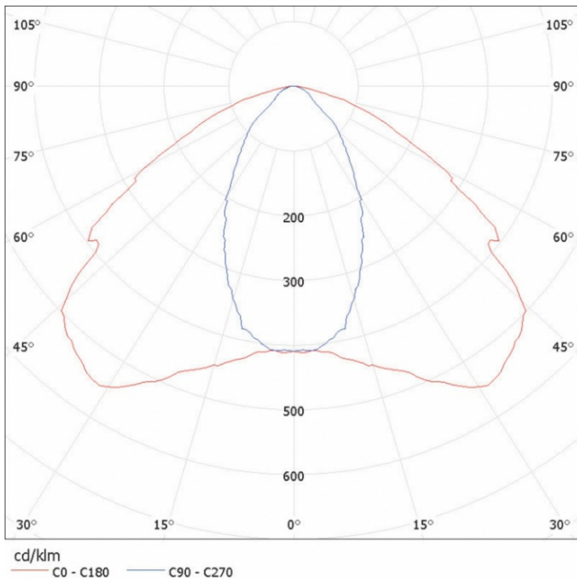
PRIMOS LED5 (450lm)
