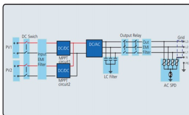
Growatt 3-6kTL3-S topologia
