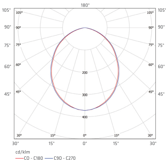
DL 185 SMD LED 21W
